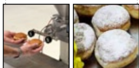
Double spout 160mm + injections 60 Pieces/min.
